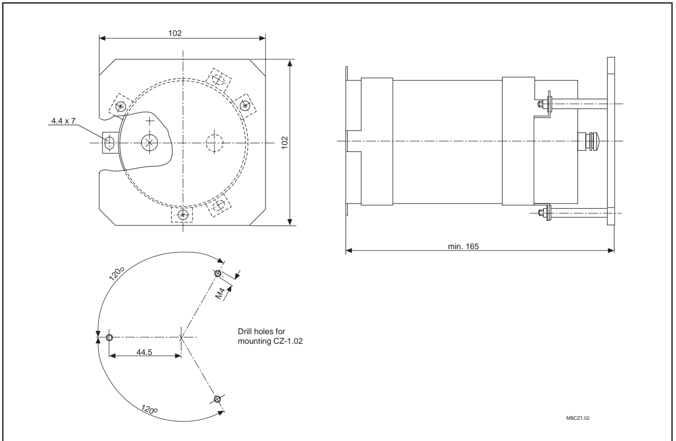
Figure 7.4: Dimensional data for the CZ 1.02 additional capacitor
