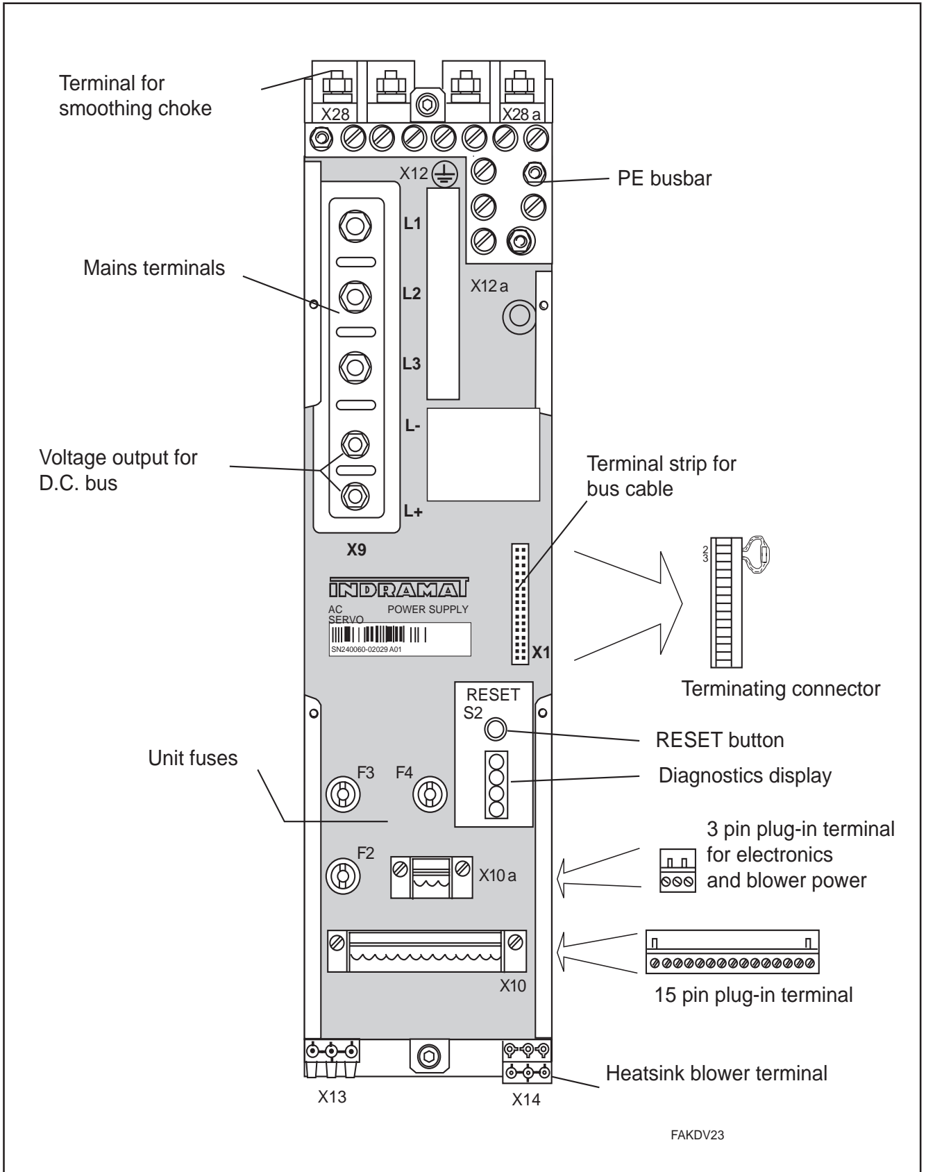
Figure 3.11: KDV 2.3 from the front
