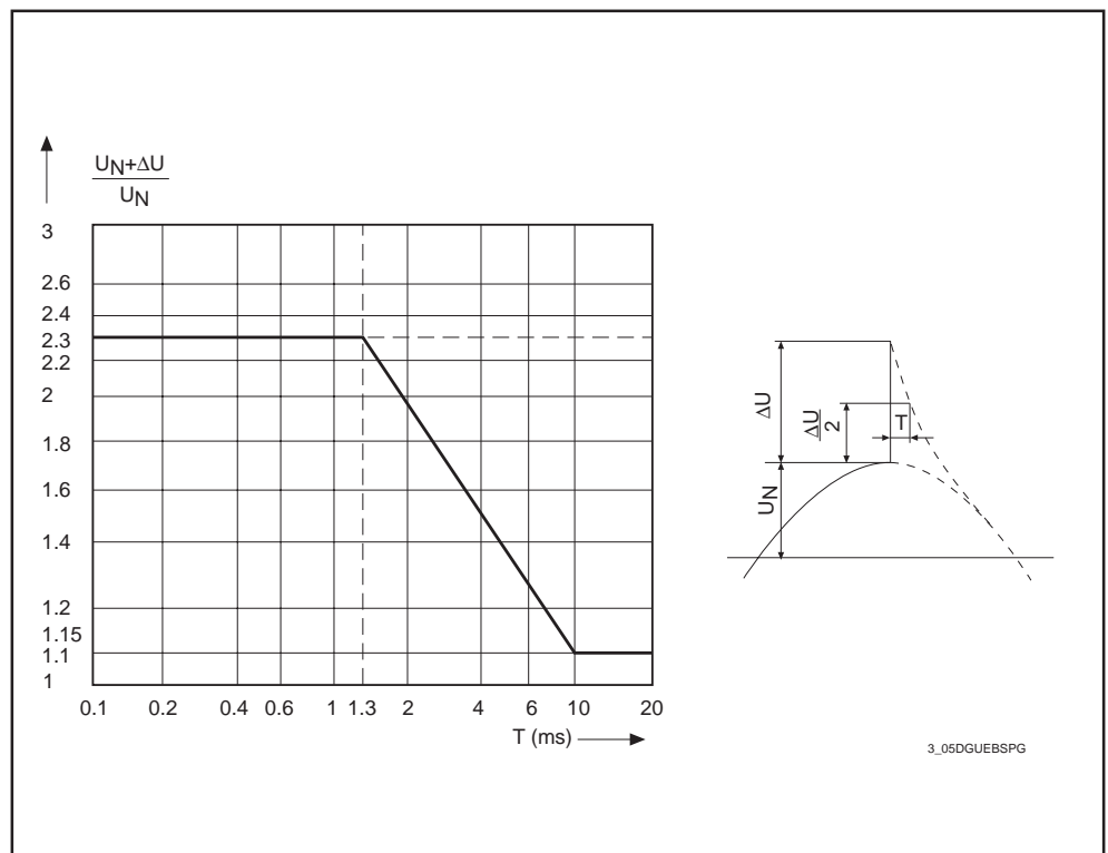
Figure 3.6: Permissible non-periodic overvoltages per VDE 0160
