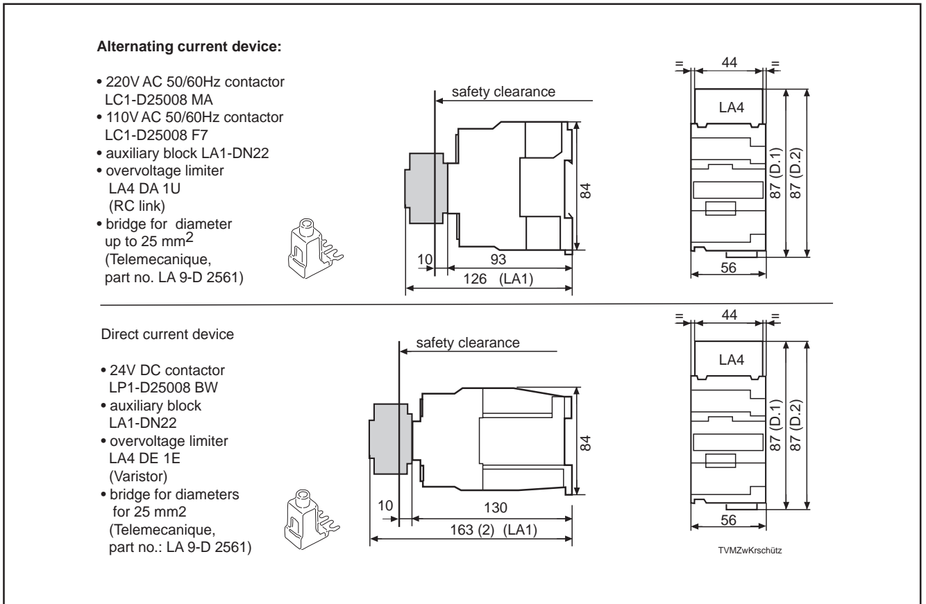
Figure 7.7: Dimensional data for dynamic brake contactor
