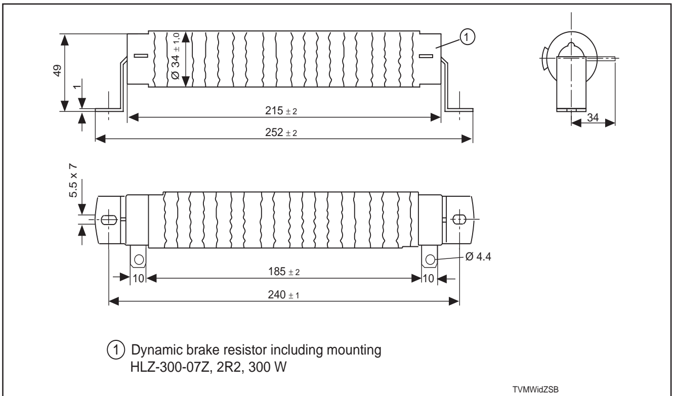
Figure 7.8: Dimensional data for dynamic brake resistor
