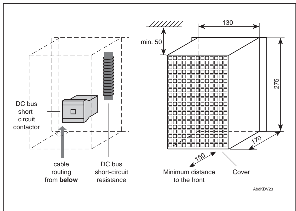
Fig. 4.3: Suitable covers and unit arrangements for the DC bus short-circuit
