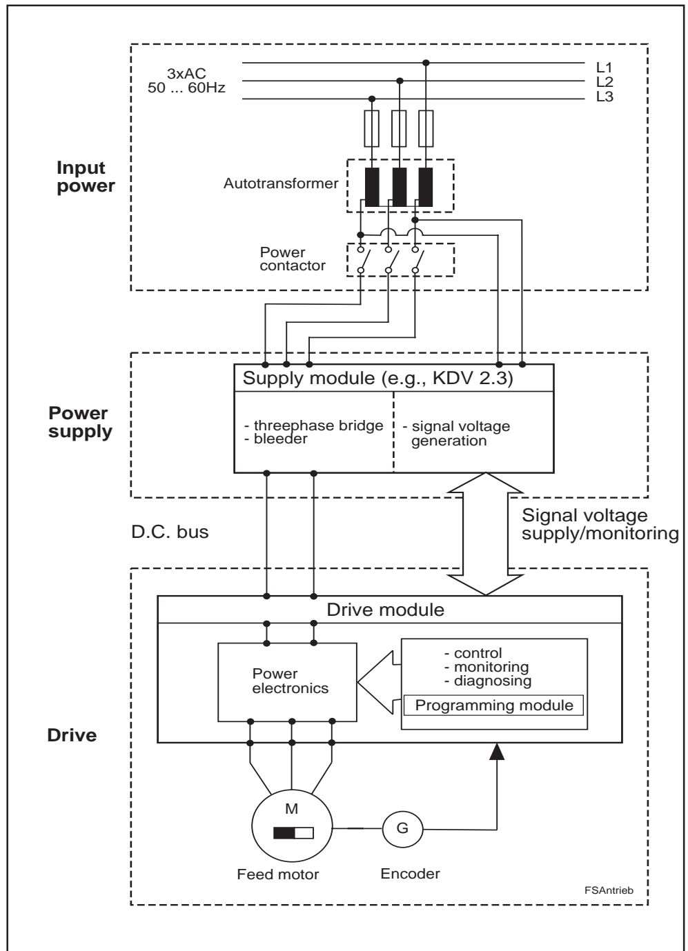
Figure 1.1: The KDV 2.3 supply module as a part of INDRAMAT's AC drive system
