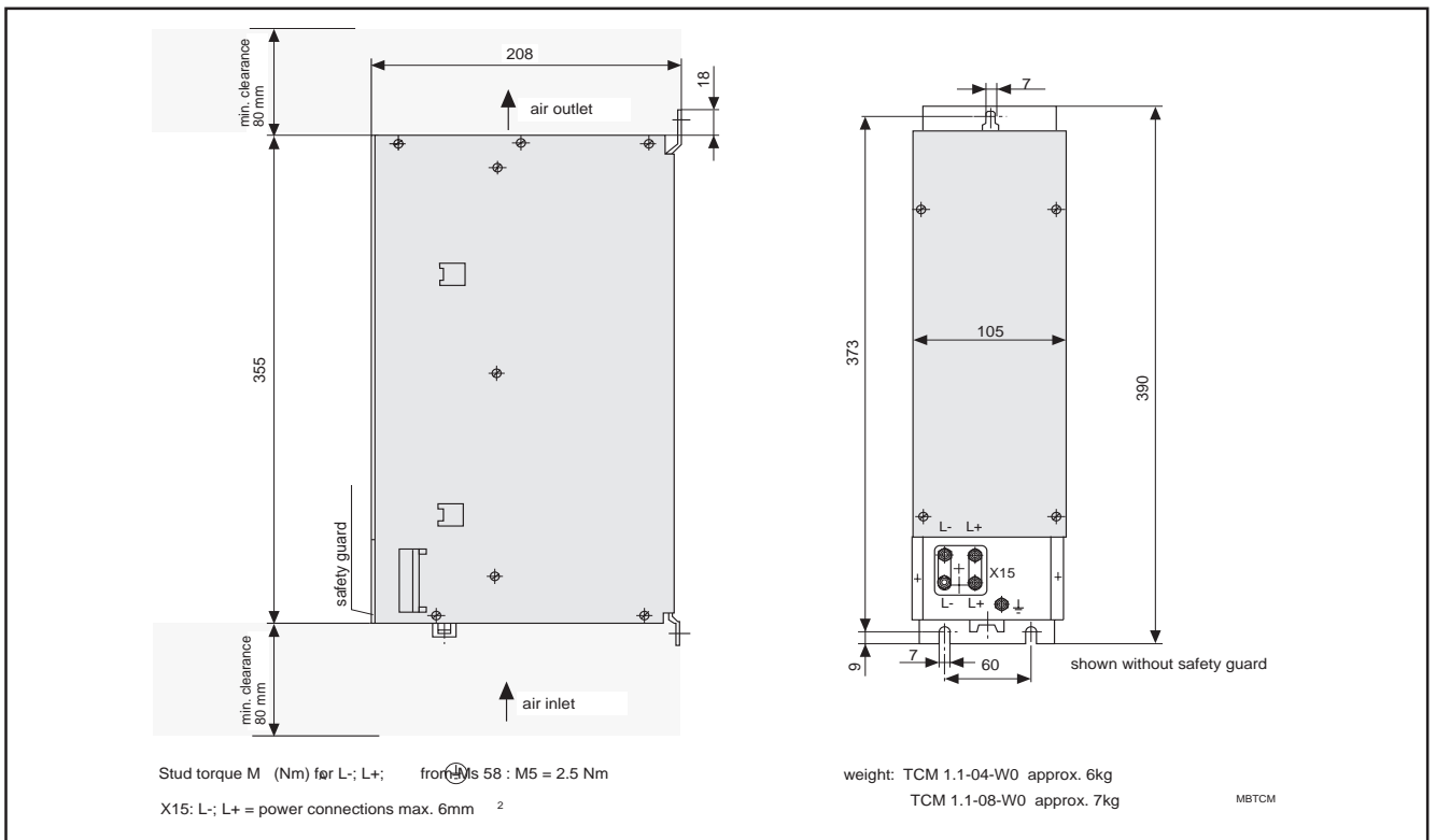
Figure 7.5: Dimensional data for the TCM additional capacitor module
