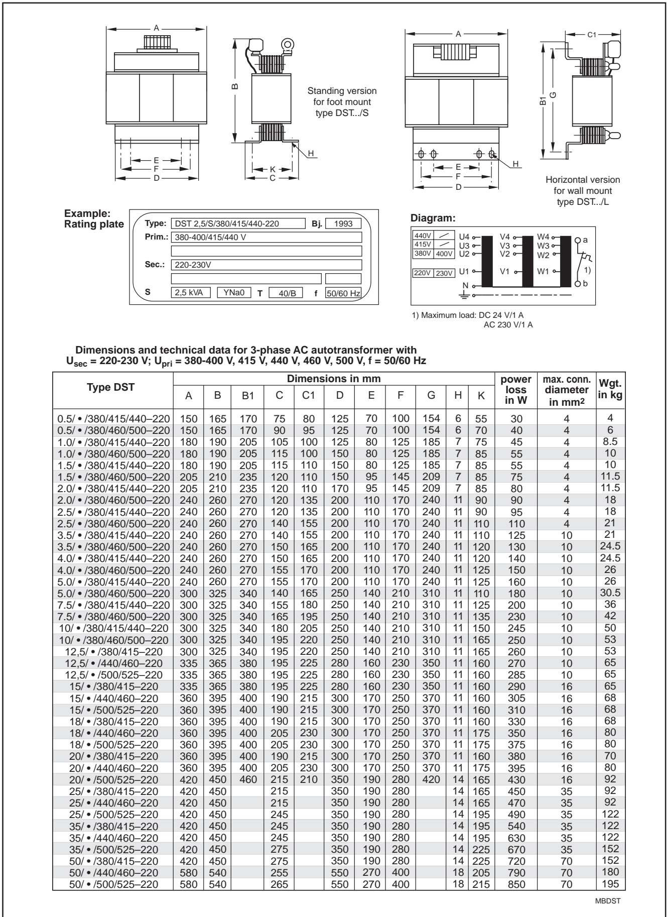
Figure 7.2: Dimensional data of the DST threephase AC autotransformer
