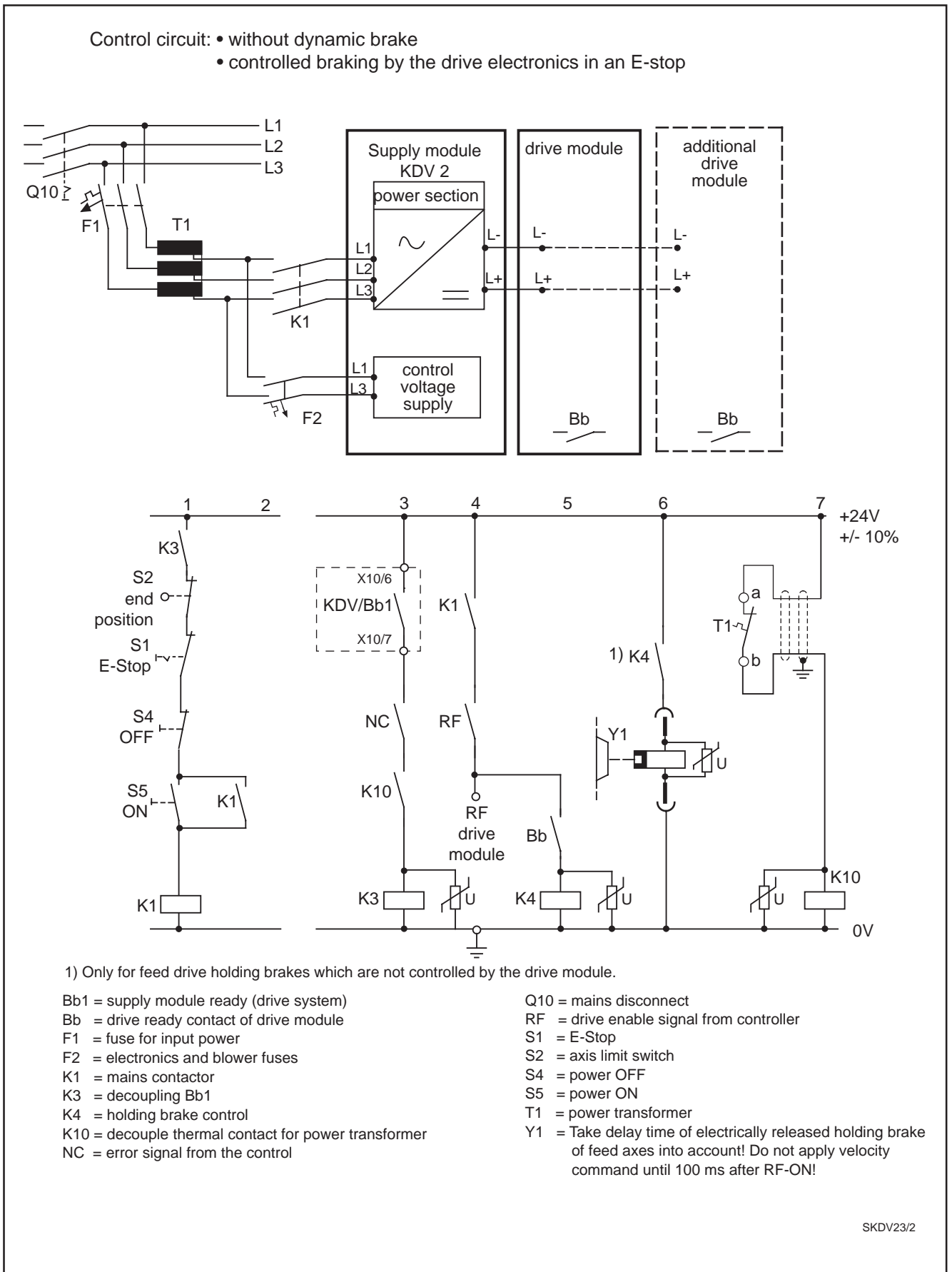
Figure 4.5: Control circuits for KDV 2.3 without dynamic braking
