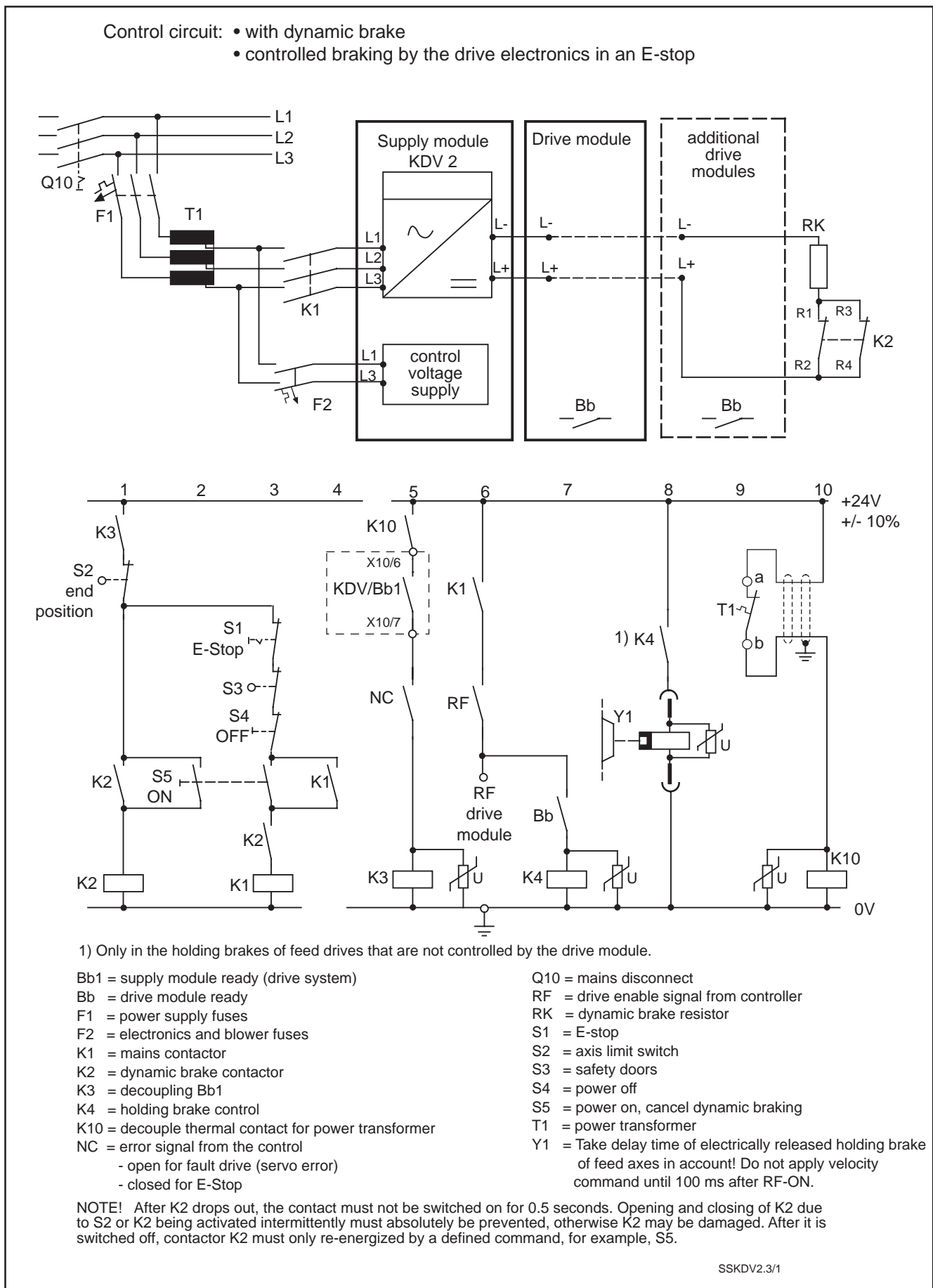
Figure 4.4: Control circuits without soft-start resistor with dynamic braking
