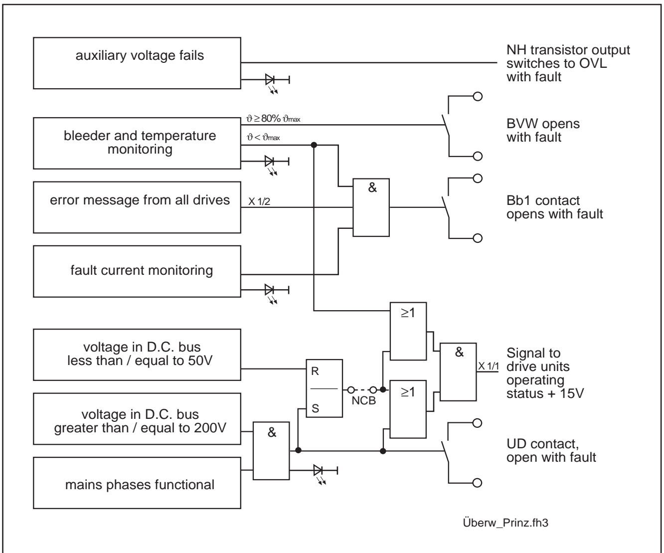
Figure 5.3: Diagram of interfaces for monitoring and diagnostics systems
