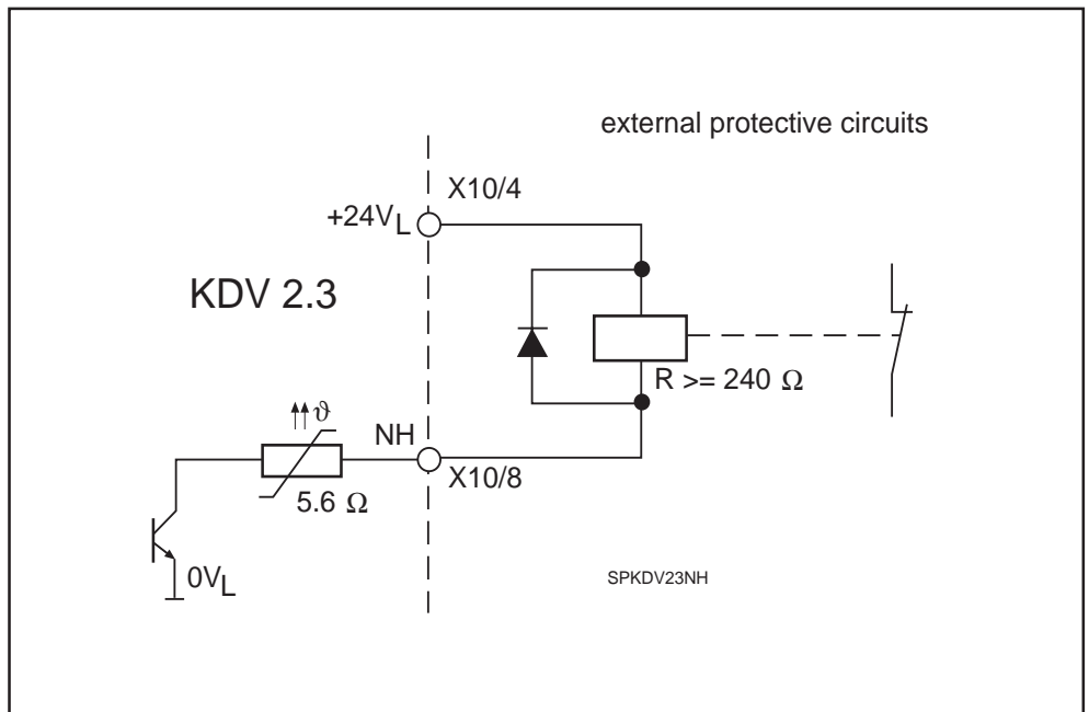
Figure 5.2: Protective circuit of the NH transistor output
