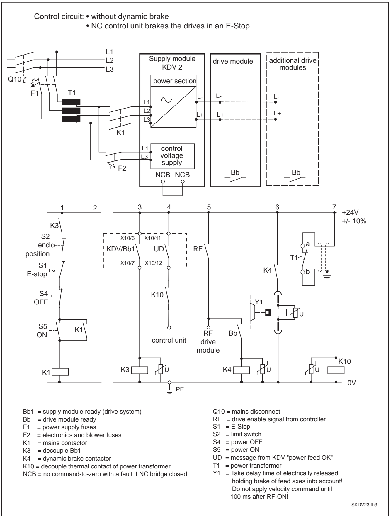
Figure 4.6: Control circuits for a controlled braking with an E-Stop or power failure
