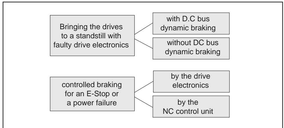
Figure 4.1: Differentiating features of the power circuits
