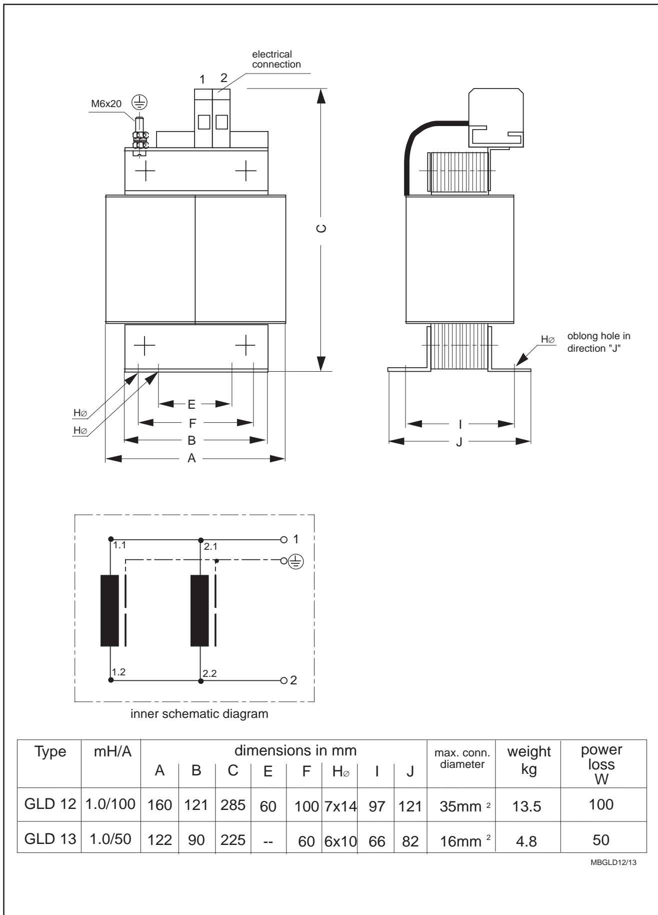
Figure 7.6: GLD 12/13 smoothing choke - dimensional data
