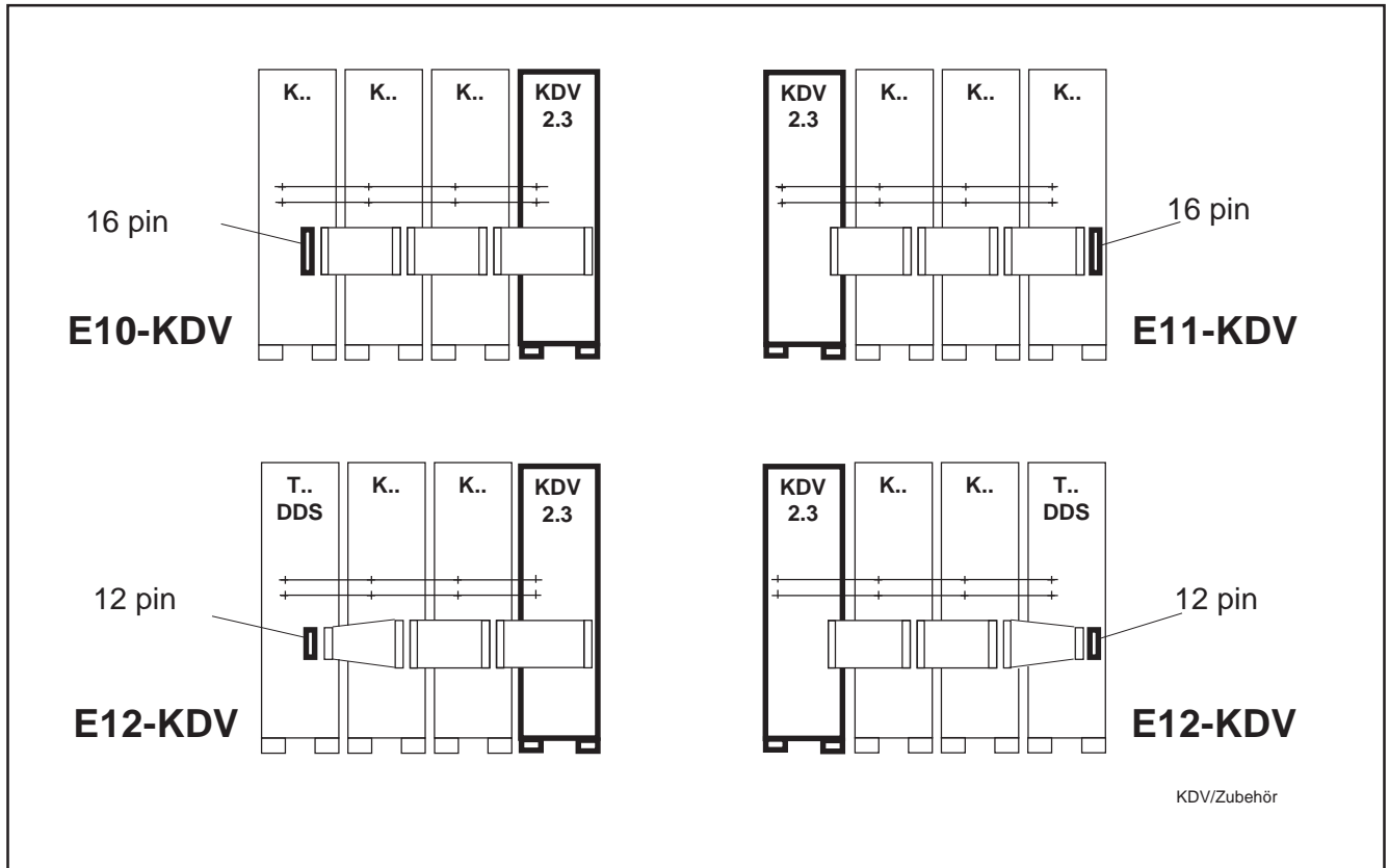
Figure 8.3: Summary of electrical connecting accessories
