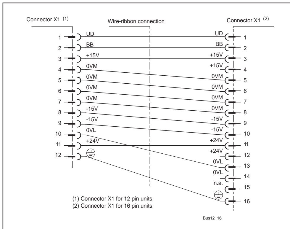
Figure 3.9: Wire-ribbon for transition from 12-pin to 16-pin connector
