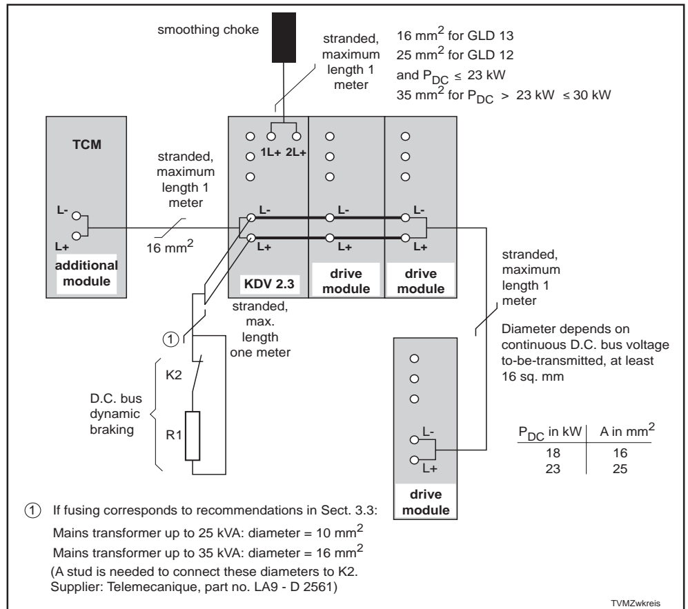
Figure 3.7: DC bus wiring
