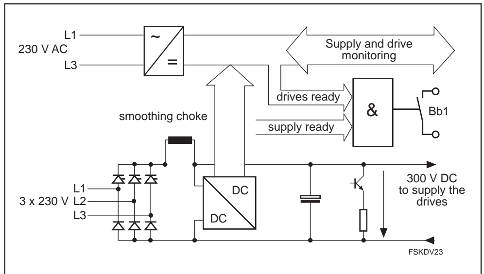
Figure 1.2: The design of the KDV 2.3 supply module
