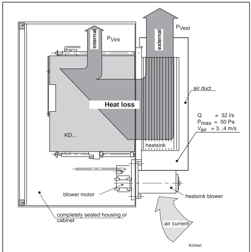
Figure 3.14: A break down of the heat losses
