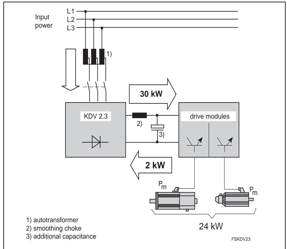
Figure 2.1: Power range of a KDV 2.3 supply module
