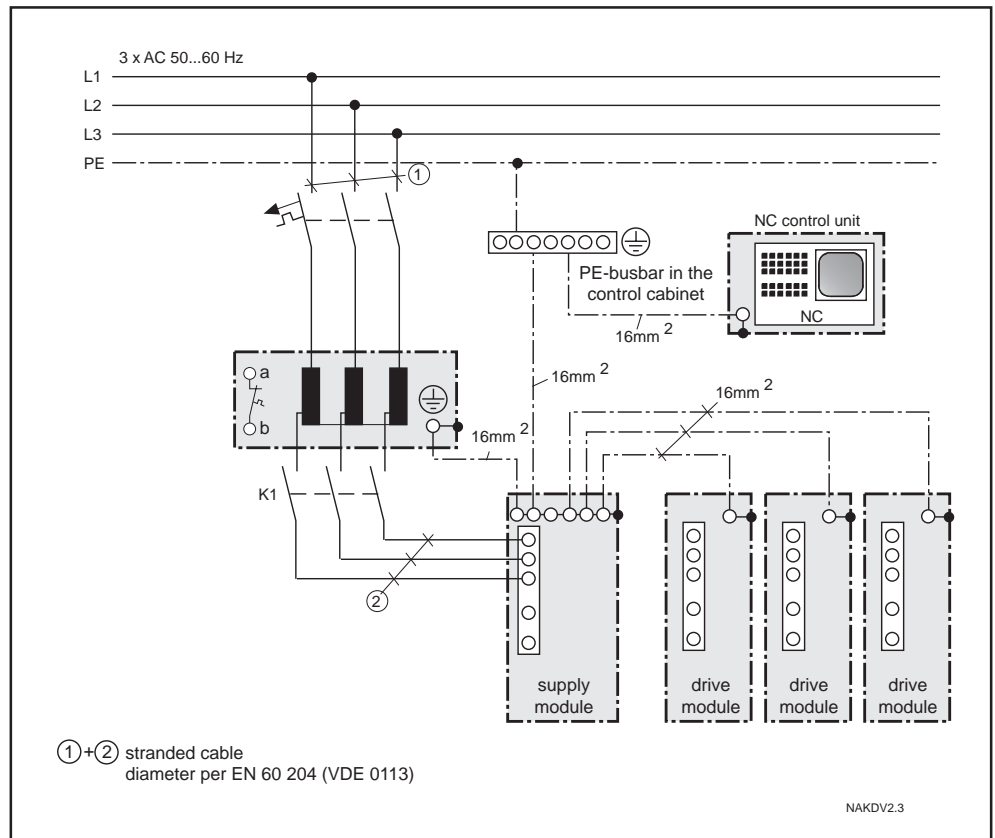
Figure 3.2: Connecting the KDV 2.3 to the mains via an autotransformer
