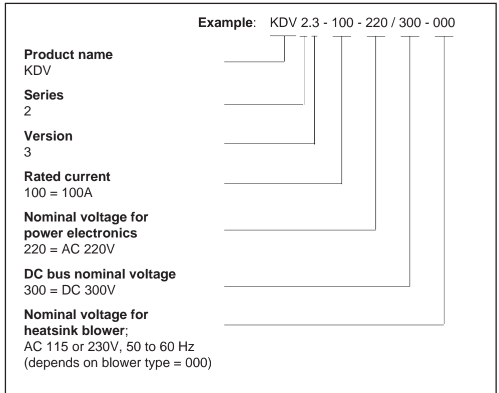
Figure 8.1: KDV type keys
